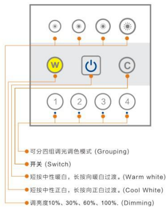
LED 调光调色触摸控制面板 CCT and Dimming Control Panel
